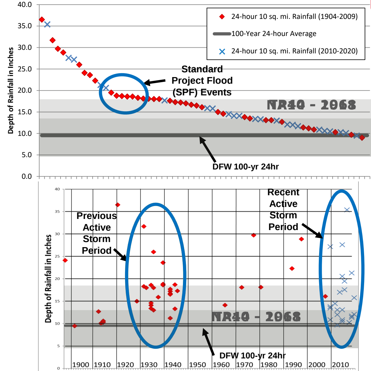
24 Hour Rainfall for 10 Sq. Mi.
